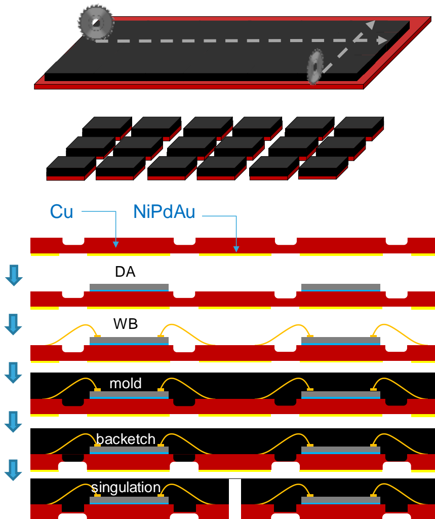
Fig. 1. Schematic of conventional mechanical blade singulation, and the package assembly flow. DA – die attach; WB – wirebond.
